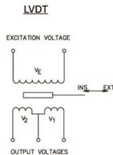
Electrical Schematic
