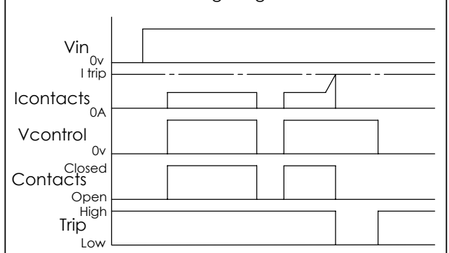
Timing Diagram
